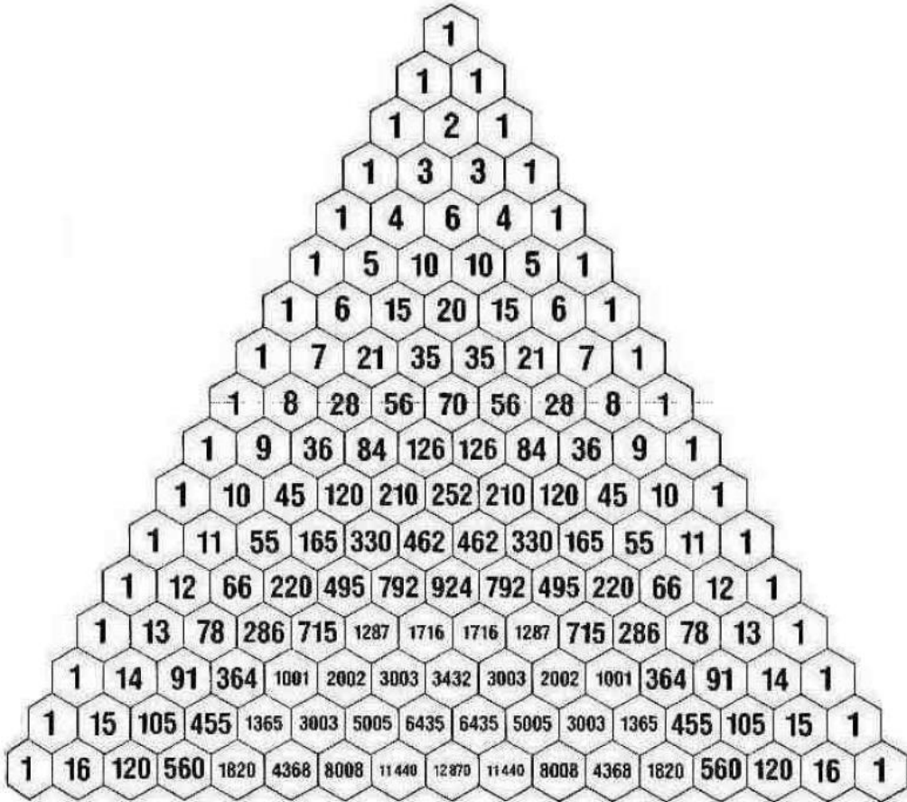
Pascal's Triangle. Multiples of 3
