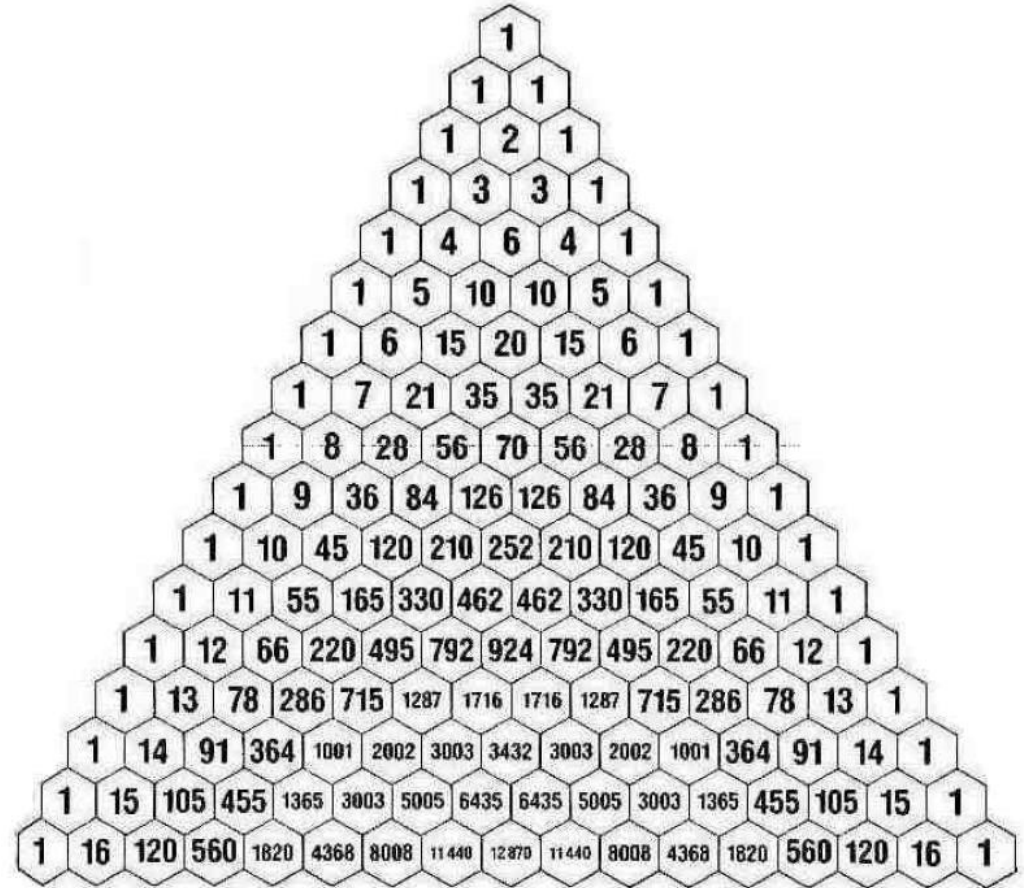
Pascal's Triangle. Multiples of 4
