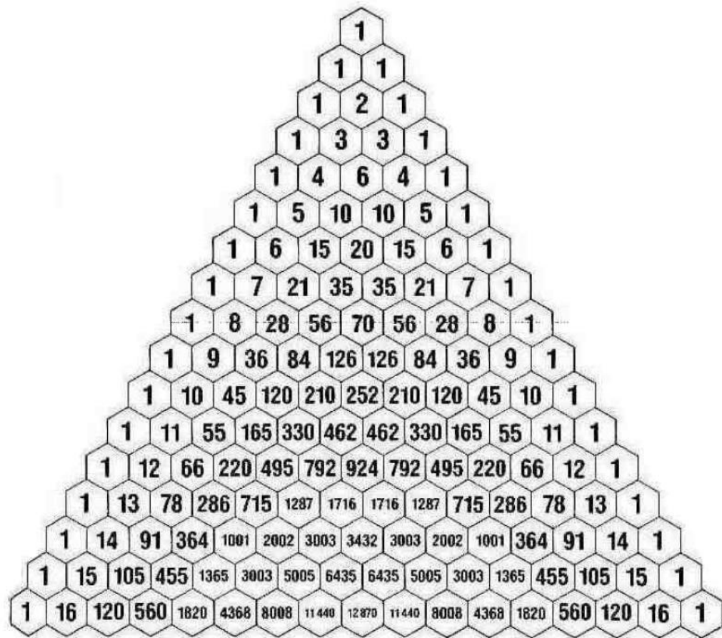
Pascal's Triangle. Multiples of 5
